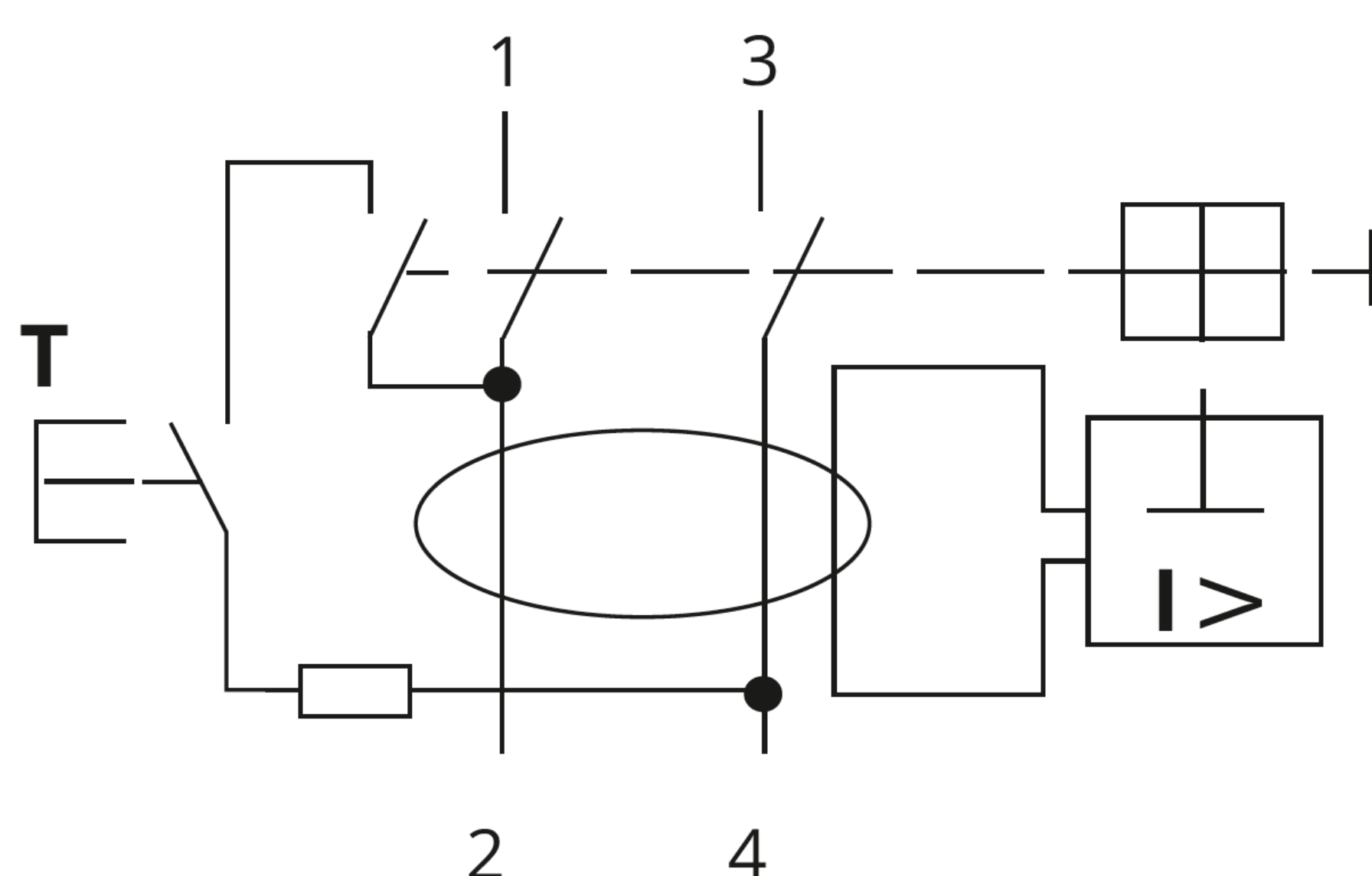
TWO-POLE
