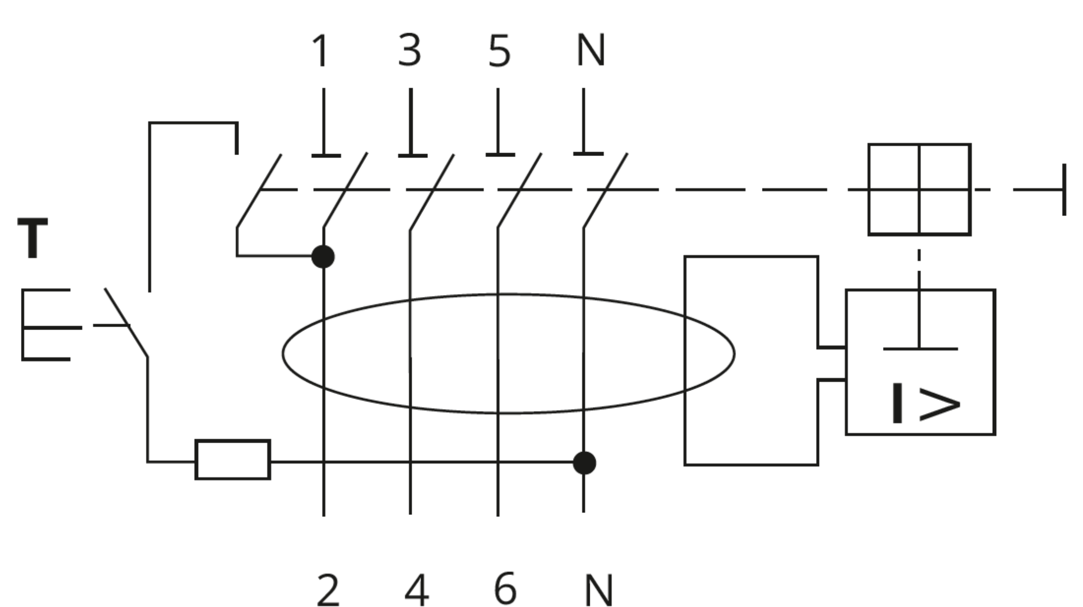
FOUR-POLE
