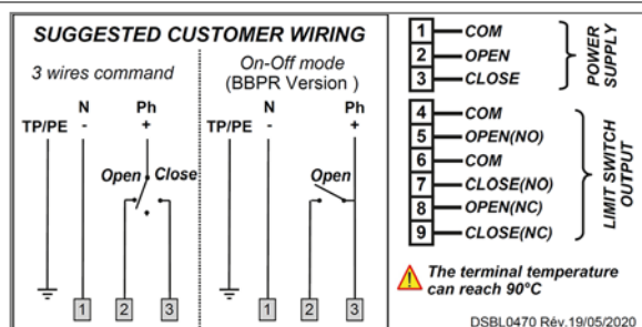
VR/VS multivolt (except POSI)
