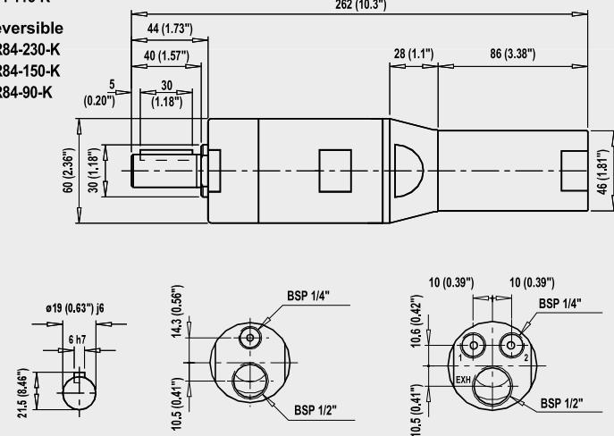
Non reversible
