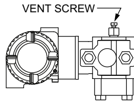
Figure 8 - Vertical Mounting – Cavity Venting, and Self-Draining into Process Line
