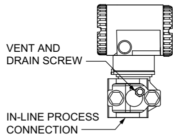
Figure 11 - Low Profile (LP1) Transmitter – Upright Mounting
