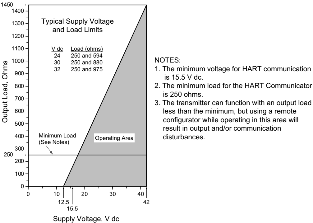
Figure 19 - 4 to 20 mA Output Supply Voltage vs Output Load
