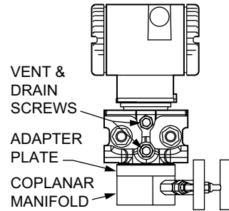
Figure 17 - Low Profile (LP2) Transmitter – Mounted to an Existing Coplanar Manifold Using Adapter Plate
