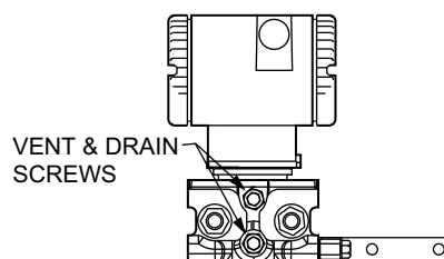
Figure 16 - Low Profile (LP2) Transmitter – Shown on a Coplanar Bracket
