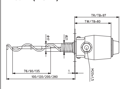
LR 80. ... (TR/TW)
