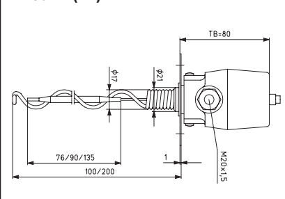
LR 80.2.. (TB)
