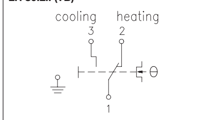
LR 80.2.. (TB)
