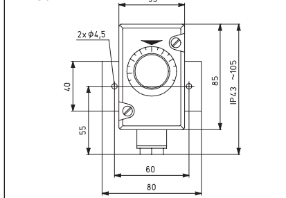
LR 80....
