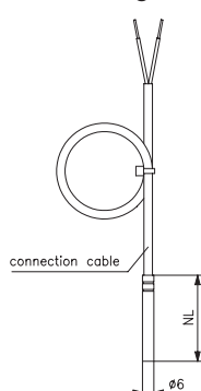
Dimension drawing
