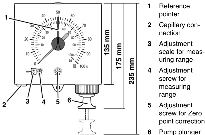
Fig. 1: Front view Unitel
