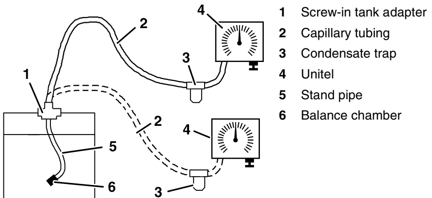
Fig. 4: Installing capillary line
